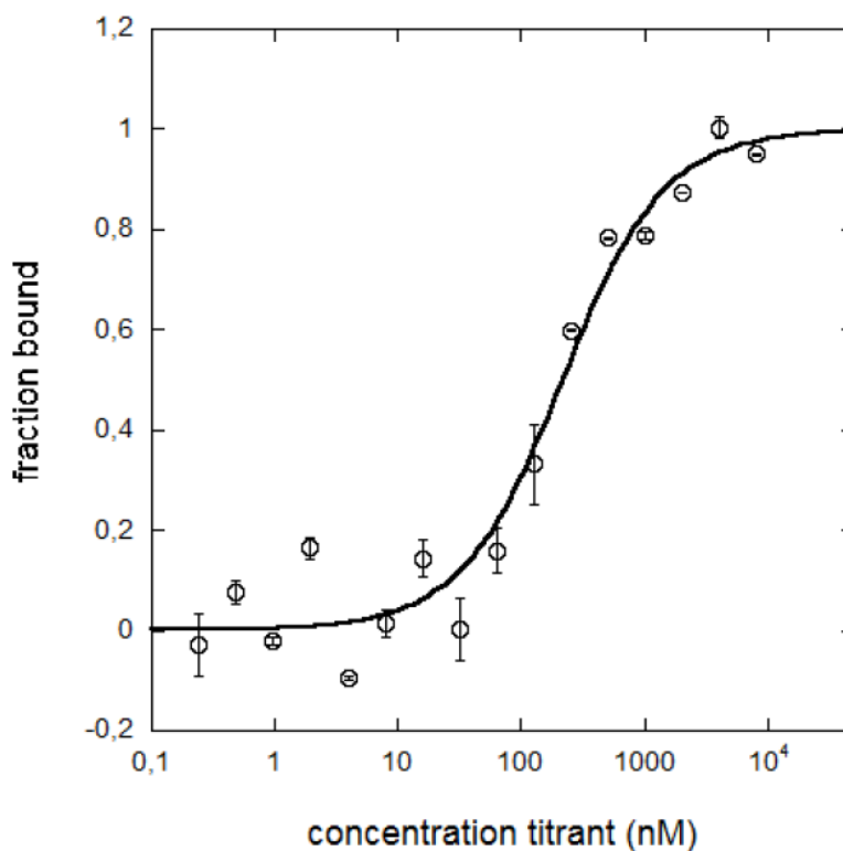
Figure 1. Aptamer-HSA binding. The fraction of bound aptamer is plotted versus the titrated target concentration, R^2 = 0.965 .
